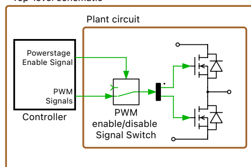
Top-level schematic
